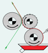
Flexographic printing
