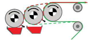
3-roller combi coating system
