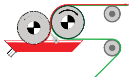
Engraved roller system
