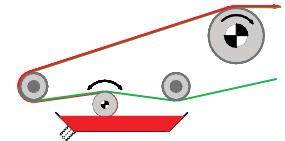
Micro roller coating system
