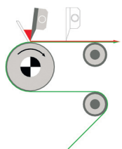
Knife system
